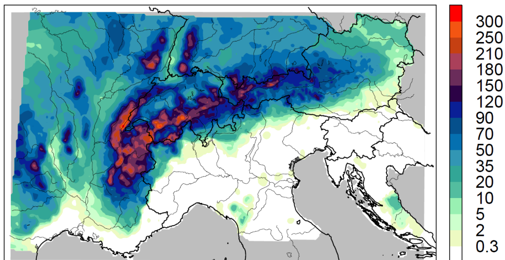
Figure 1: Two-day precipitation total for an episode of heavy precipitation in the Alps in mm (13.2-14.2.1990).
