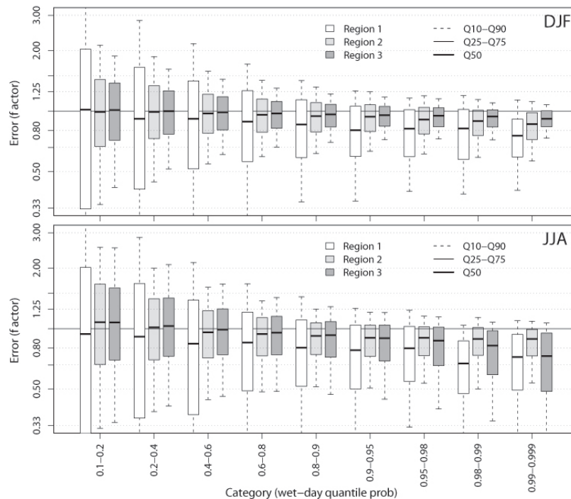
Figure 2. Boxplot of interpolation errors determined from a systematic leave-one-out crossvalidation in three characteristic regions. Region 1: area with a coarse station network, Region 2: mountainous area with a dense network, Region 3: flatland area with a dense network. Errors are expressed as the ratio between the interpolation (at the location of the station) and the observation at the station. The errors are stratified into bins of precipitation intensity defined in terms of quantiles (wet days only) with low (high) intensities on the left (right). The upper plot is for winter (DJF), the lower for summer (JJA). The boxplots represent the median (bold line), the inter-quartile range (box) and the 10-90% quantile range (whisker) of the error distribution. From Isotta et al. (2014).
